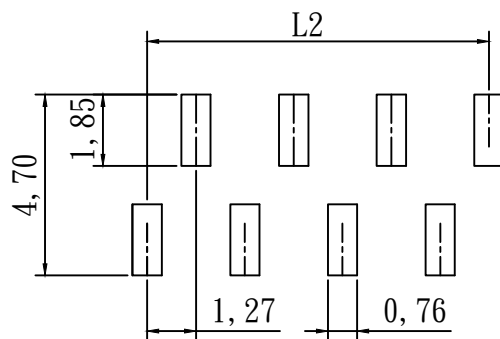
RECOMMENDED P. C. B. LAYOUT (TB)
