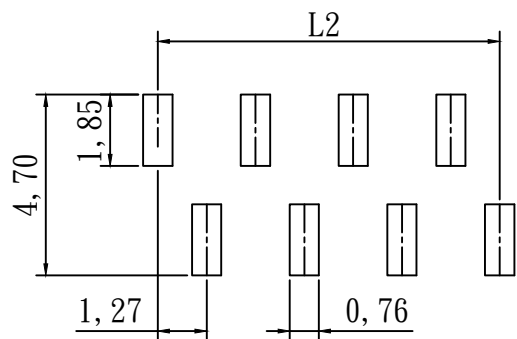
RECOMMENDED P. C. B. LAYOUT (TA)
